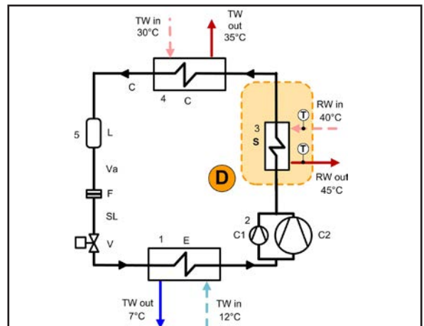
D - Partial recovery device TW in chilled water inlet TW out chilled water outlet 1 - Internal exchanger 2 - Compressors 3 - Recovery exchanger (D) 4 - External exchanger 5 - Expansion electronic valve RW in - Recovery water input RW out - Recovery water output T - Temperature probe
